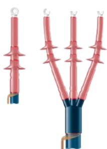
11kV Outdoor
