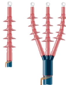
33kV Outdoor
